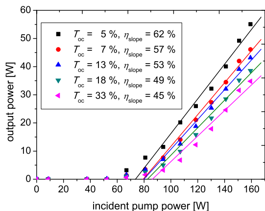
Fig. 5 CW laser performance of the 52-mm long Ho(1%):YAG rod at room temperature
