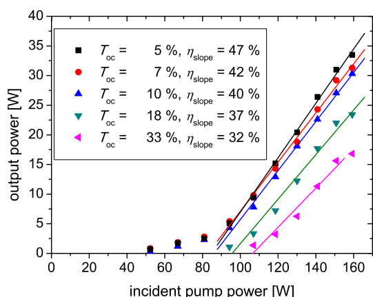
Fig. 6 CW laser performance of the 52-mm long Ho(0.5%):YAG rod at room temperature
